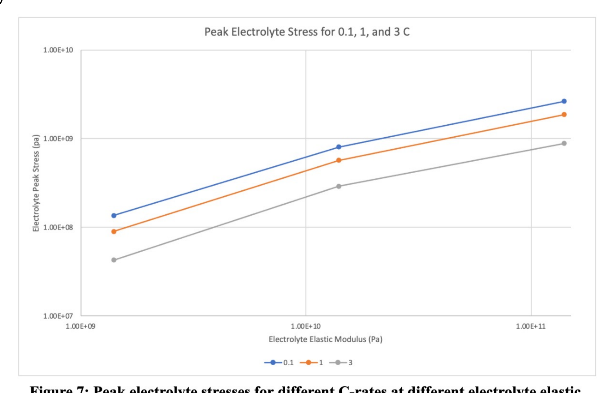
Figure 7: Peak electrolyte stresses for different C-rates at different electrolyte elastic moduli
