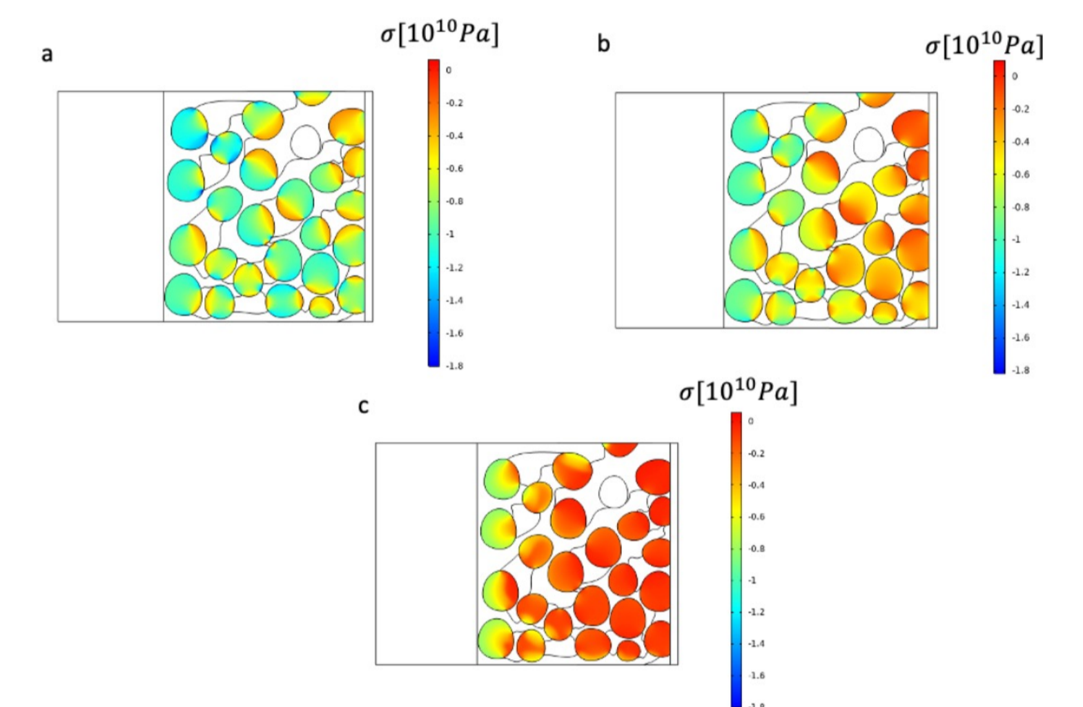
Figure 4: Particle stress with electrolyte Young's modulus of 140 GPa with C rates of 0.1C (a), 1 C (b) and 3 C (c)
